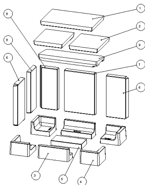
Abb. 23: Keramott 63x40x42
