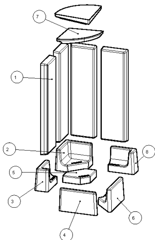
Abb. 21: Keramott 38x38x57
