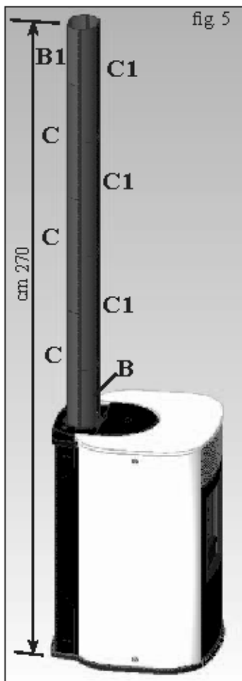
Detail of assembly of pipe cover elements
